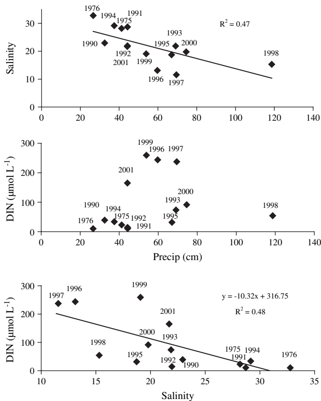
Fig. 11. Average rainy season salinity versus annual precipitation (cm) (top panel), average rainy season DIN ( \mu\text{mol L}^{-1} ) versus annual precipitation (cm) (middle panel), average rainy season DIN ( \mu\text{mol L}^{-1} ) versus average rainy season salinity (bottom panel) from the 10 km station in 1975–1976 and 1990–2001.
