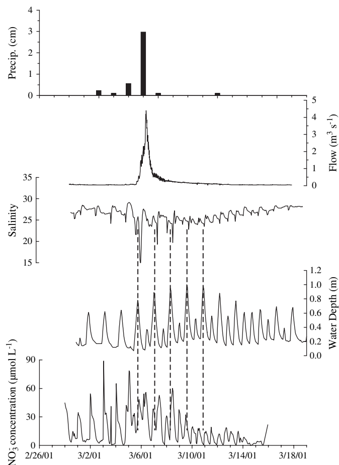
Fig. 7. Daily precipitation (cm), Carneros Creek flow ( \text{m}^3 \text{s}^{-1} , from Los Huertos et al., 2001), salinity, water depth (m), and \text{NO}_3^- concentrations ( \mu\text{mol L}^{-1} ) in Azevedo Pond, 26 February to 18 March, 2001. Dashed vertical lines indicate high tides that coincide with either low salinity or high \text{NO}_3^- concentrations.
