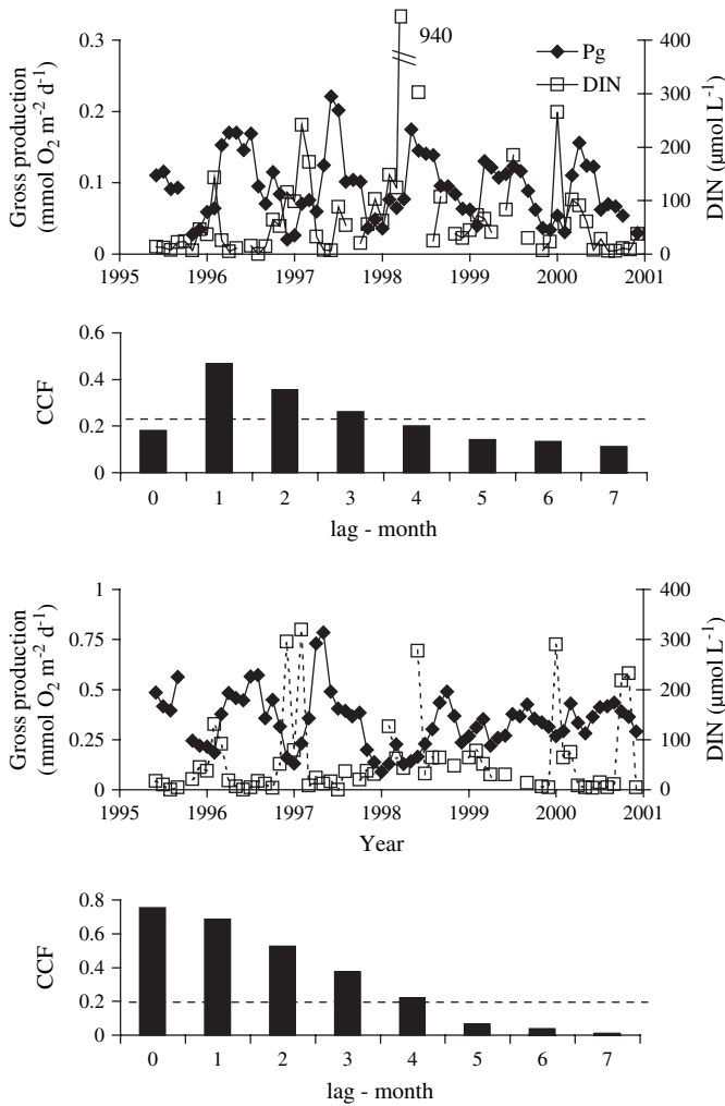
Fig. 4. Gross primary production (Pg) ( \text{mmol O}_2 \text{ m}^{-2} \text{ d}^{-1} ) and DIN concentrations ( \mu\text{mol L}^{-1} ) between May 1995 and December 2000 in South Marsh (top panel), Cross-correlation function (CCF) for primary production and DIN at monthly lag intervals for South Marsh (second from top panel). Azevedo Pond gross primary production (Pg) ( \text{mmol O}_2 \text{ m}^{-2} \text{ d}^{-1} ) and DIN concentrations ( \mu\text{mol L}^{-1} ) between May 1995 and December 2000 (second from bottom panel). Cross-correlation function (CCF) for primary production and DIN at monthly lag intervals for Azevedo Pond (bottom panel). 95% confidence interval shown by dashed line.
