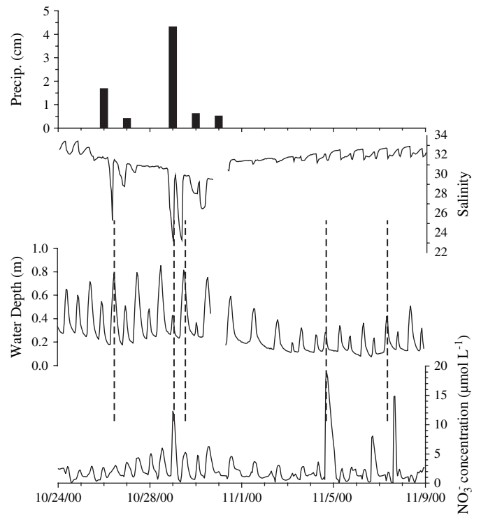
Fig. 6. Daily precipitation (cm), salinity, water depth (m) and \text{NO}_3^- concentrations ( \mu\text{mol L}^{-1} ) in Azevedo Pond, 24 October to 9 November, 2000. Dashed vertical lines indicate high tides that coincide with either low salinity or high \text{NO}_3^- concentrations.
