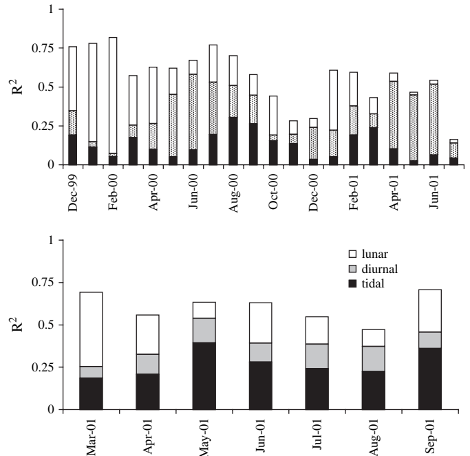
Fig. 5. R^2 values obtained from harmonic regression models of log transformed \text{NO}_3^- data from Azevedo Pond (top panel) in 2000 and 2001 and Main Channel (bottom panel) in 2001.
