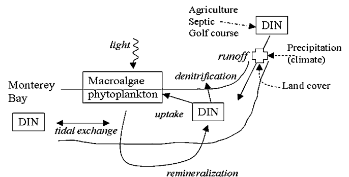
Fig. 10. Conceptual model highlighting the dominant factors controlling DIN concentrations in Elkhorn Slough.
