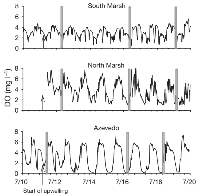
Fig. 3. Dissolved oxygen ( \text{DO} ; \text{mg l}^{-1} ) in South Marsh, North Marsh and Azevedo Pond. Arrow: start of upwelling. Vertical boxes: time of sampling. Dates are mo/d
